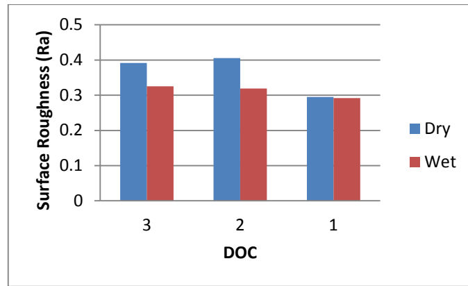
Figure 5: Surface roughness comparison between dry and wet machining for 100m/min cutting speed
