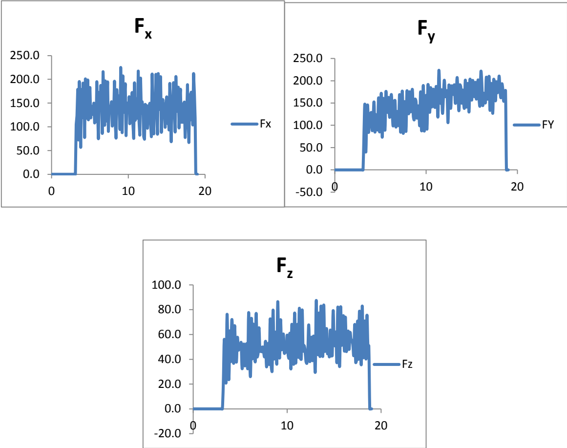
Figure 2: Cutting force in x, y and z axis for 3mm DOC, 60 m/min cutting speed
