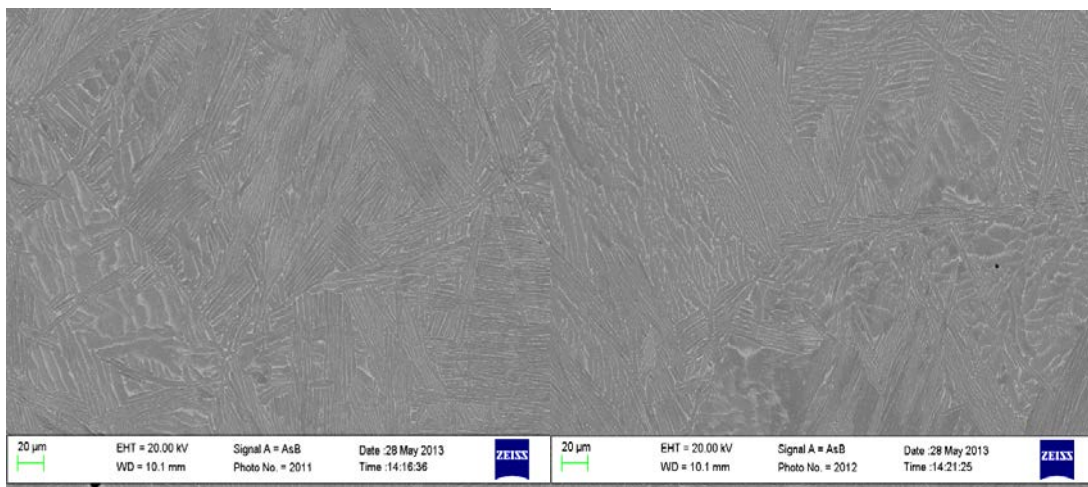
Figure 6: SEM microstructure of machined Ti-6Al-4V alloy
