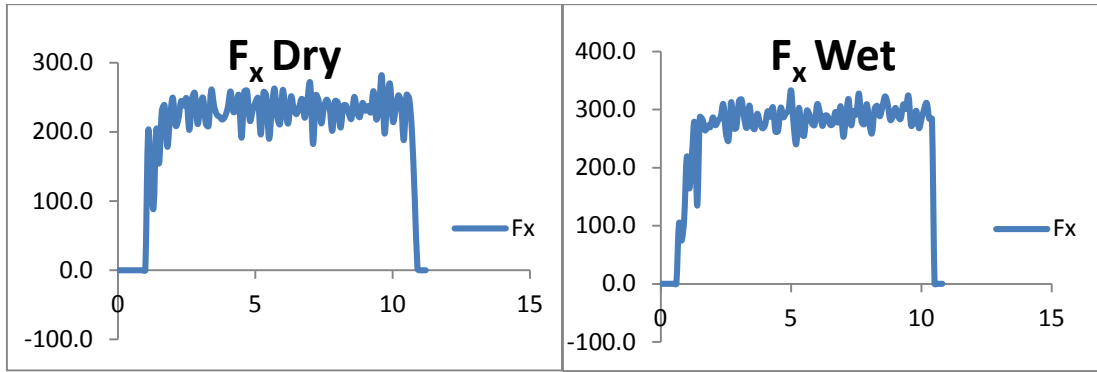
Figure 3: Cutting forces in x axis for 3mm DOC, 100 m/min
