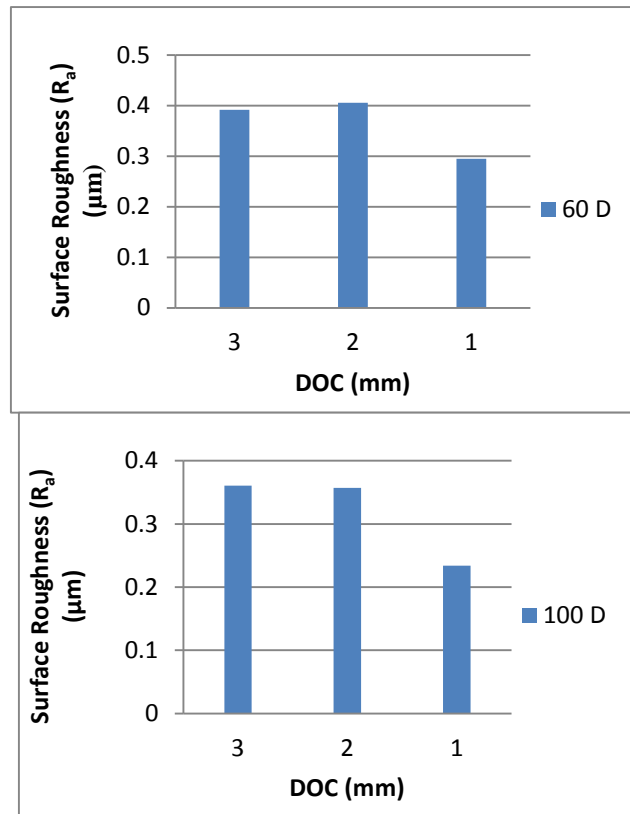
Figure 4: Surface roughness for 60m/min and 100m/min cutting speeds, dry machining
