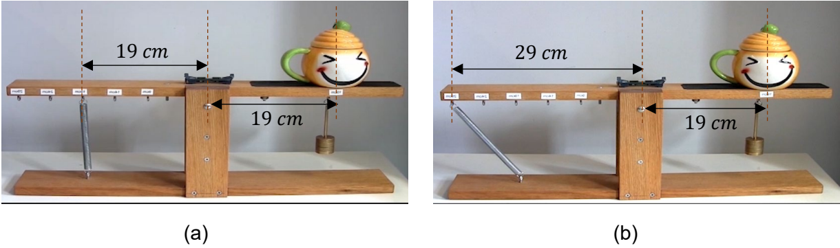
Figure 1: Two configurations of the Spring Scales experimental set-up
